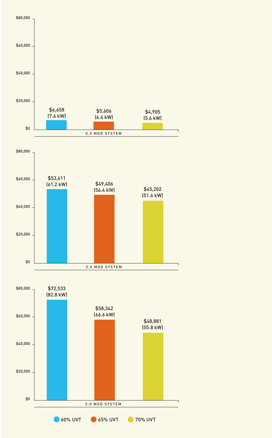
Figure 2: Annual Power Consumption For Different Levels Of UVT In Three Different Size Systems Source: Aquionics, Inc. 2014
