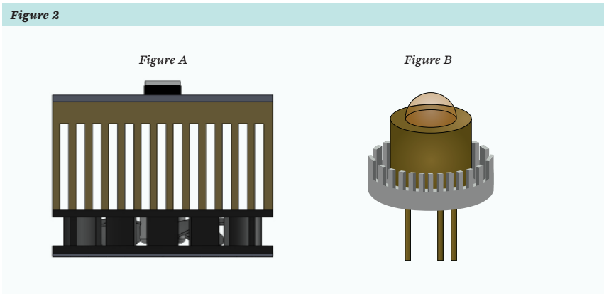
Schematic of heat sink placement for Crystal IS surface mount (a) and through hole (b) packages.
