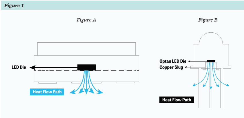
Schematic of heat flow path for Crystal IS surface mount (a) and through hole (b) packages.
