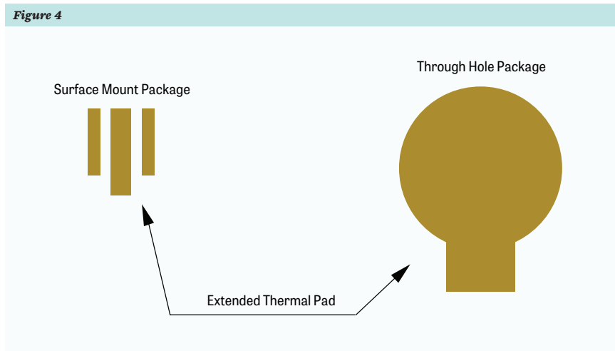
Suggested solder pattern showing extended thermal pad for measuring the solder point temperature.
