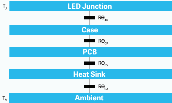
A simplified description of the thermal model for a Crystal IS LED package attached to a heat sink.
